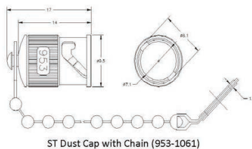
ST Dust Cap with Chain (953-1061)
