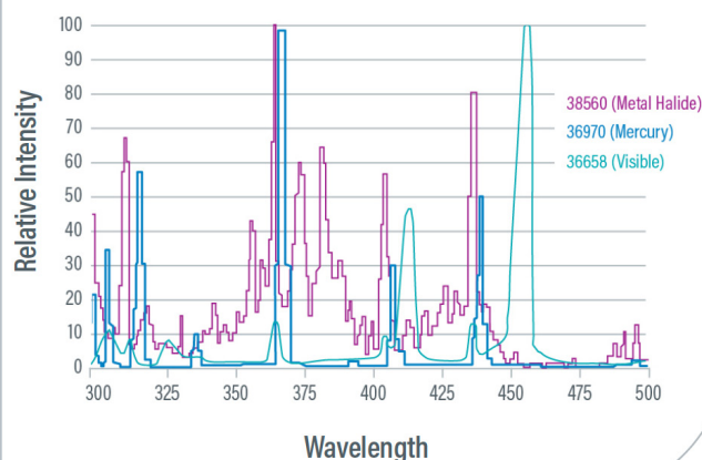
Spectral Outputs for Dymax 400W Flood Bulbs
