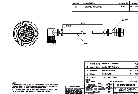
Cable, FX1250, 2M Type I to L
