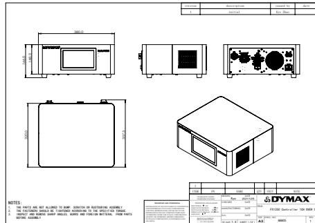
FX1250 Controller 1CH OVER SIZE
