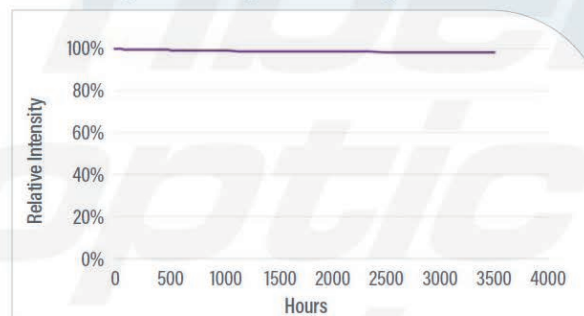
Figure 6. LED Degradation Testing - PrimeCure®
