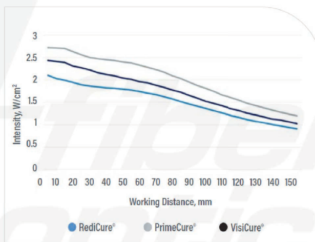
Figure 3. BlueWave® FX-1250 Intensity Over Working Distance
