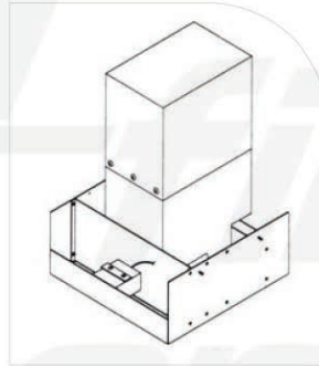
One center-mounted Fusion F300 6" wide single exposure
