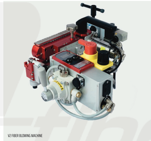
V2 FIBER BLOWING MACHINE
