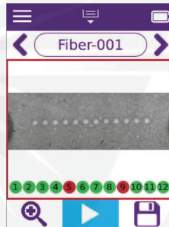
Wide FOV of an MPO end face
