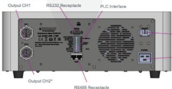
Figure 3 2CH Controller Back Panel
