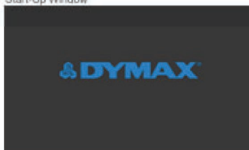
Figure 23. Start-Up Window
