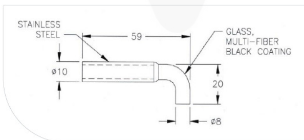
Figure 13. 5-mm, 90° Terminator (PN 38049)
