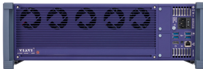
Figure 2 - MAP-380 rackmount and benchtop mainframes, rear view
