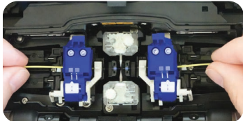
Dual Fiber Loading
