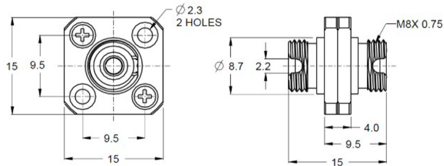
FC Square Adapter Screw Mount
