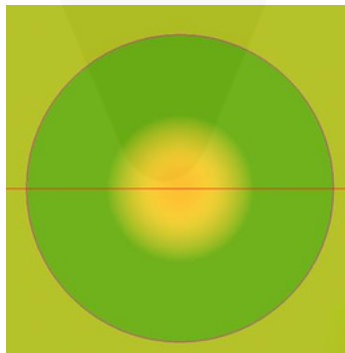
Graded index multimode fiber
