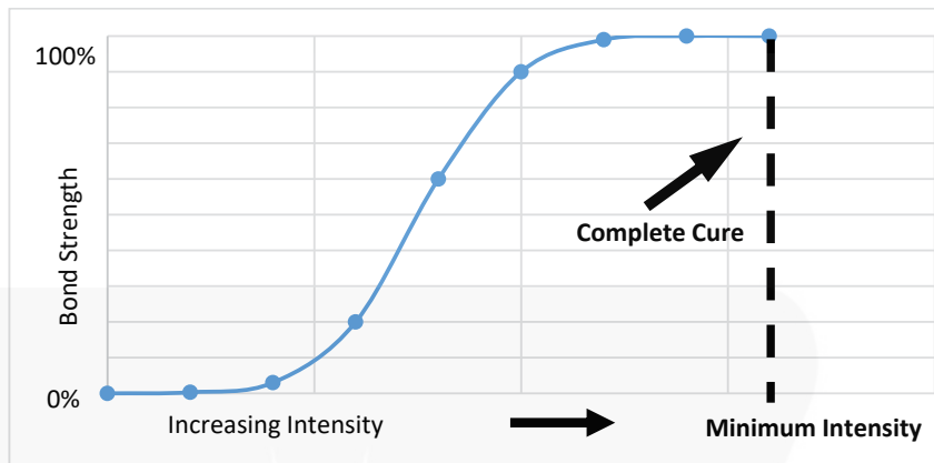
Figure 1. Curing Energy Profile (Exposure Time Held Constant)
