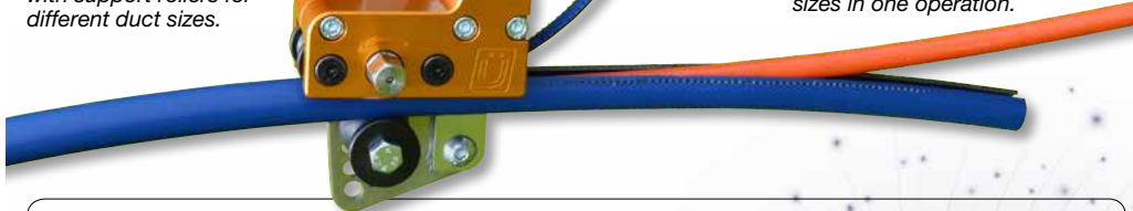
EASY FIBER DUCT SLITTER cuts a wide groove in the most commonly used duct types/sizes in one operation.
