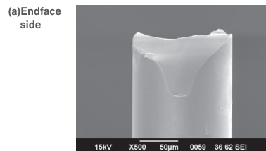
SEM images of Fiber micro crack
