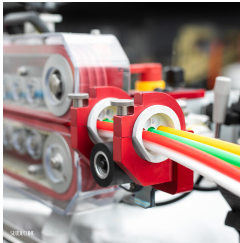
SUBDUCTING
