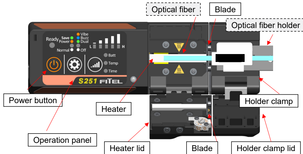
Top view (with an Optical fiber holder)
