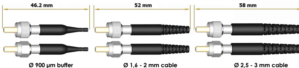
SMA 905 Crimp Type Connector Overall Dimensions
