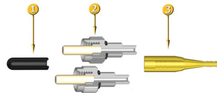
SMA 905 Crimp Type Connector for Ø 1,6 - 2 - 2,5 - 3 mm cables
