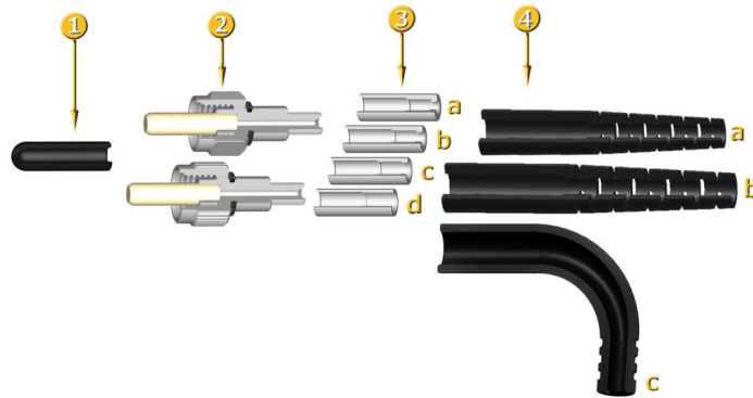
SMA 905 Connector for Ø 900 µm buffer
