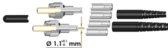
SMA 905 Crimp Type Connector for Ø 1,6 - 2 - 2,5 - 3 mm cables
