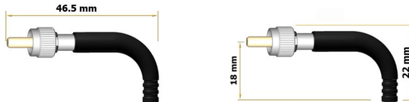
SMA 905 Crimp Type Connector with 90° Black Boot for Ø 2 - 3 mm cables
