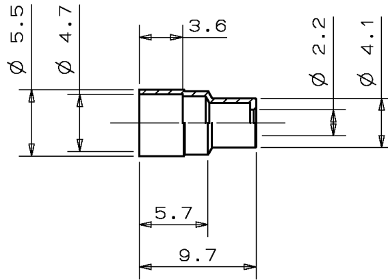
Figure 10 ③-1 Crimping Ring (for \varnothing 2 mm cord)
