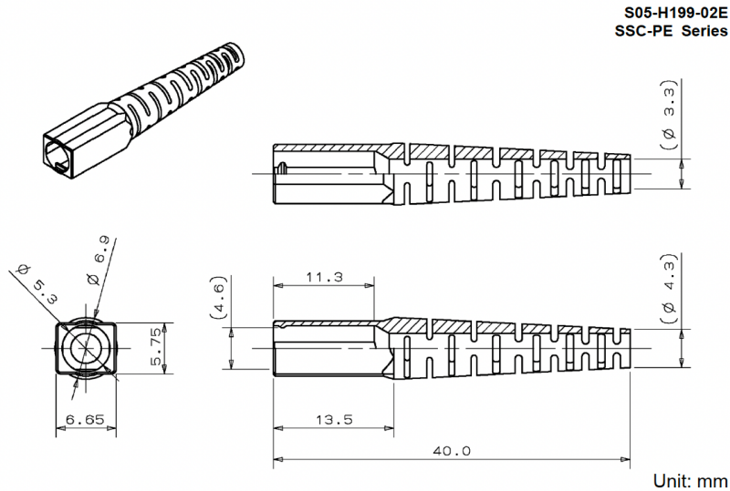
Figure 9 ④-1 Boot (for Ø 3 mm cord)
