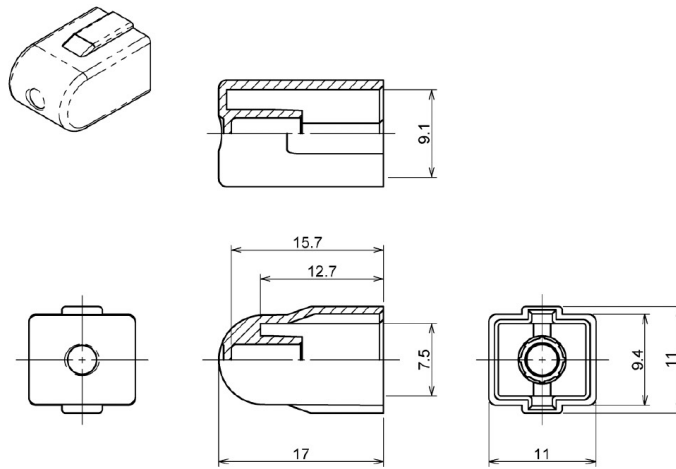
Figure 14 ⑤-2 Cap (Dust cap)
