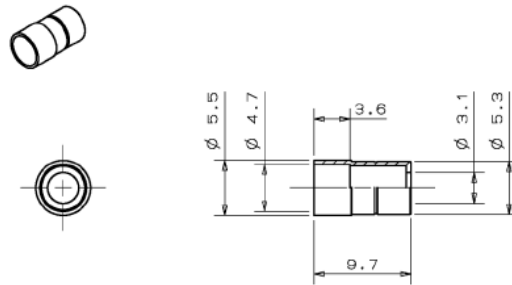
Figure 7 ③-1 Crimping Ring (for 3 mm cord)
