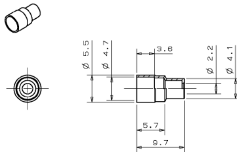
Figure 8 ③-2 Crimping Ring (for 2 mm cord)
