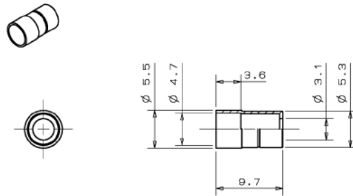
Figure 7 ③-1 Crimping Ring (for \varnothing 3 mm cord)
