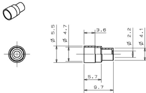
Figure 8 ③-2 Crimping Ring (for \varnothing 2 mm cord)
