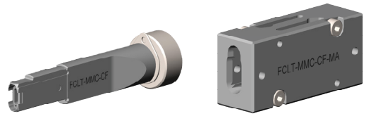
FCLT-MMC-CF: Contact free MMC cleaning tip
